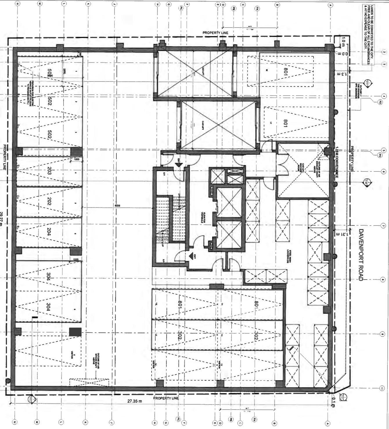
1 FLOOR PLAN LEVEL P3 1:50
