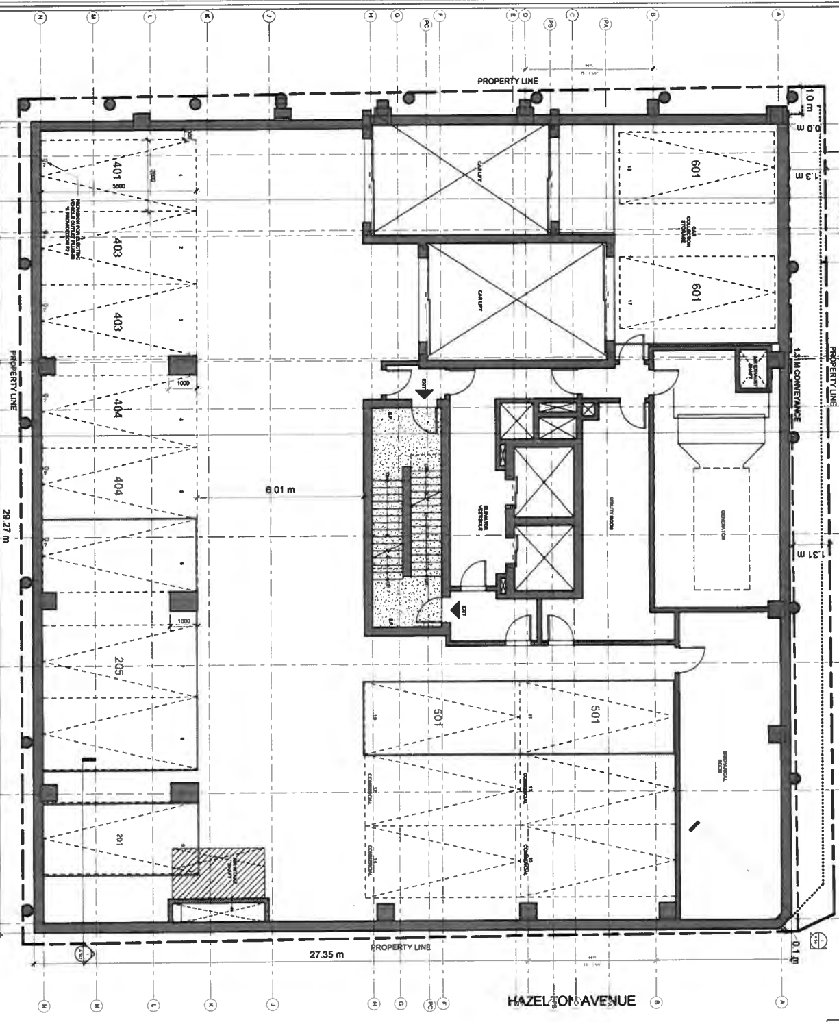
1 FLOOR PLAN LEVEL P2
